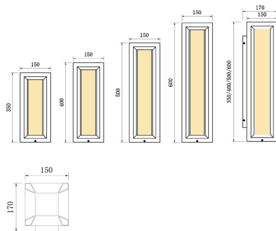
Product Dimension Drawing
