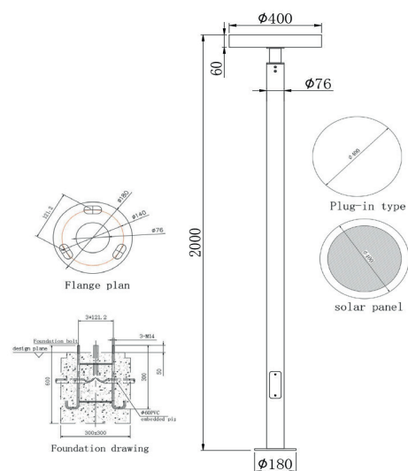
Product Dimension Drawing
