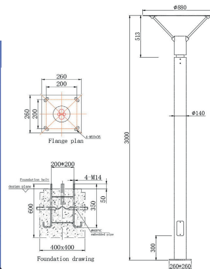
Product Dimension Drawing
