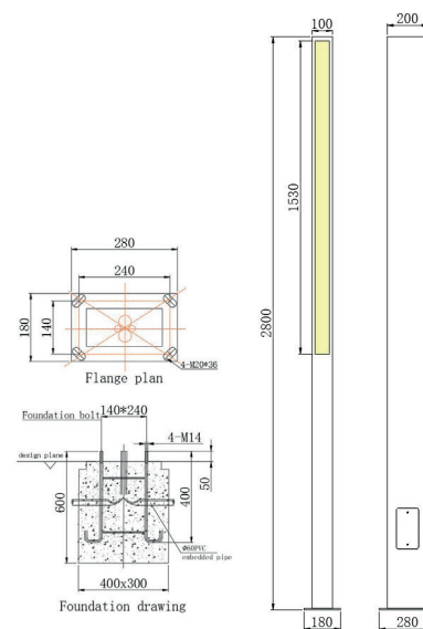
Product Dimension Drawing
