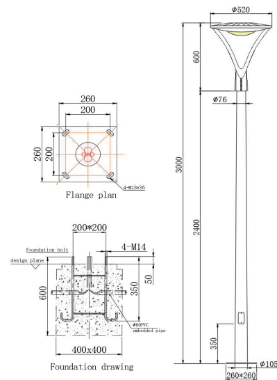
Product Dimension Drawing
