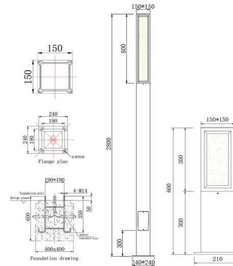
Product Dimension Drawing
