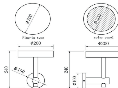
Product Dimension Drawing
