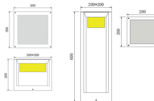
Product Dimension Drawing
