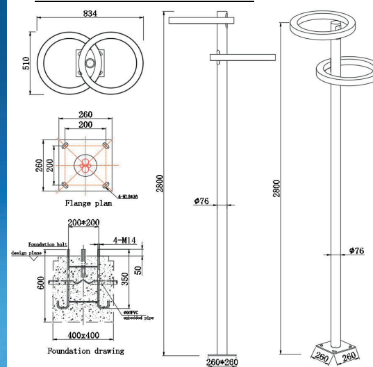
Product Dimension Drawing
