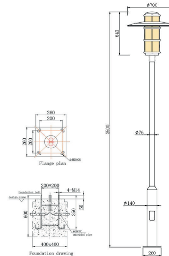
Product Dimension Drawing
