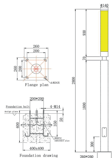
Product Dimension Drawing
