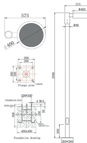
Product Dimension Drawing
