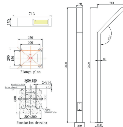
Product Dimension Drawing
