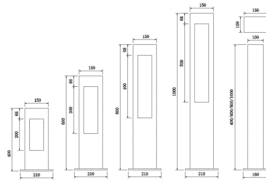
Product Dimension Drawing
