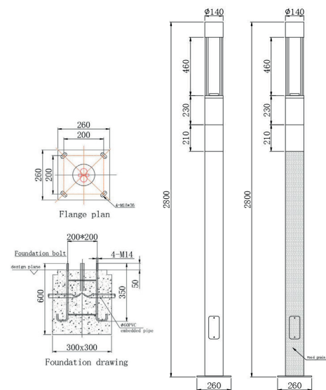
Product Dimension Drawing
