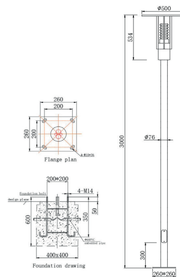
Product Dimension Drawing
