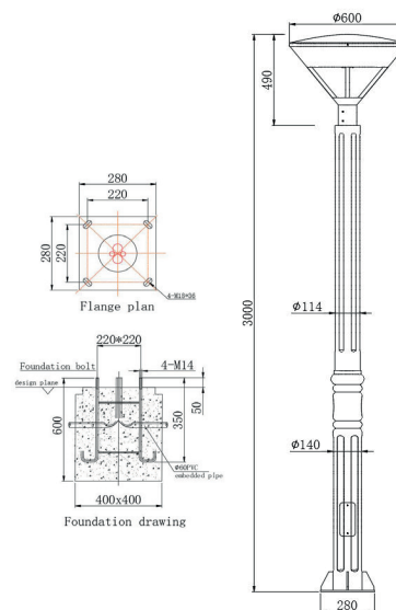
Product Dimension Drawing
