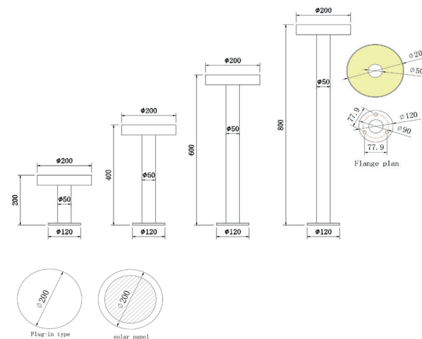
Product Dimension Drawing
