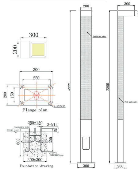
Product Dimension Drawing
