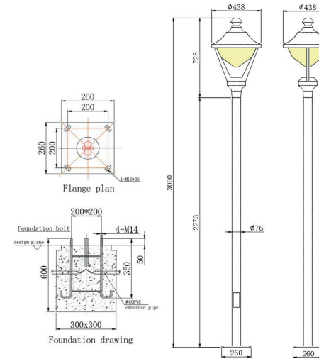
Product Dimension Drawing
