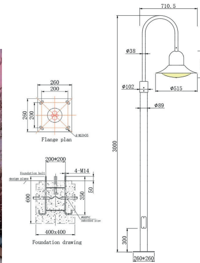
Product Dimension Drawing
