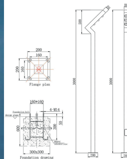
Product Dimension Drawing
